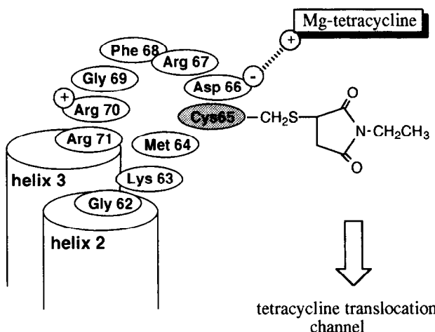
Fig. 3. Model of the steric hindrance of tetracycline translocation on modification of Cys 65 with N-ethylmaleimide. The residues constituting the putative loop 2-3 of the Cys 65 mutant TetA protein are depicted as ovals. A positive charge of a divalent cation-tetracycline complex is predicted to first interact with the negative charge of Asp 66 , and then the complex molecule enters the putative substrate translocation channel. A bulky substituent of Cys 65 may be located at the entrance of the channel and thus hinder the tetracycline translocation.
